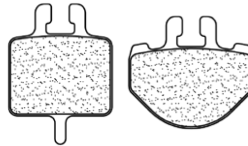
Grimeca System 1, 1.1, 7, 15
